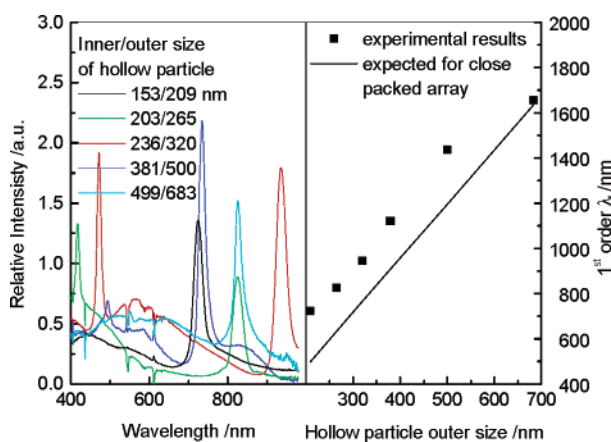
Figure 4. Bragg diffraction of close-packed colloidal crystals centrifuged from ethanol. The right-hand figure compares the observed 1st order diffraction (■) to that expected (—) for a close-packed array.
